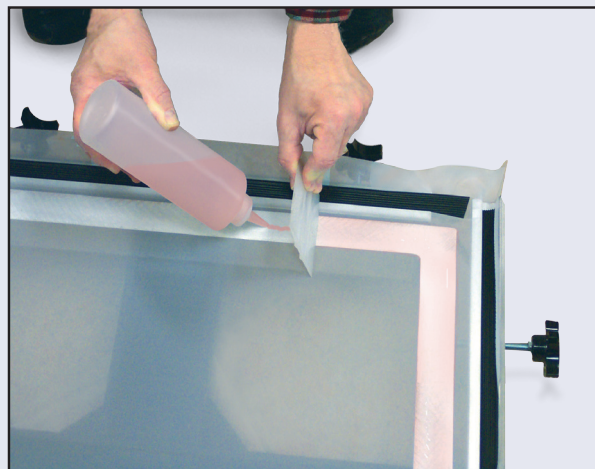
Applying Liquid Seal to bond fabric to frame. Mesh is stretched on A.W.T.'s Easy-Stretch™ manual screen stretching system.
