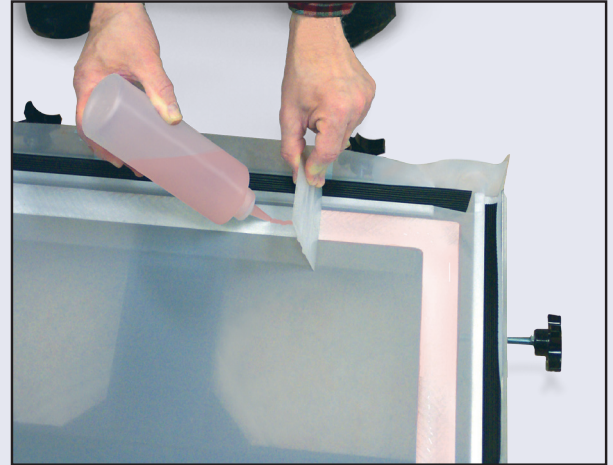
Applying Liquid Seal to bond fabric to frame. Mesh is stretched on A.W.T.'s Easy-Stretch™ manual screen stretching system.
