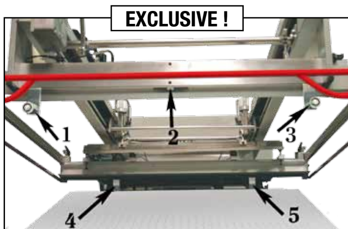
EXCLUSIVE ! Five-point masterframe lock-in: Ensures critical registration for multicolor printing. Wraparound safety bar (red) protects press operator.
